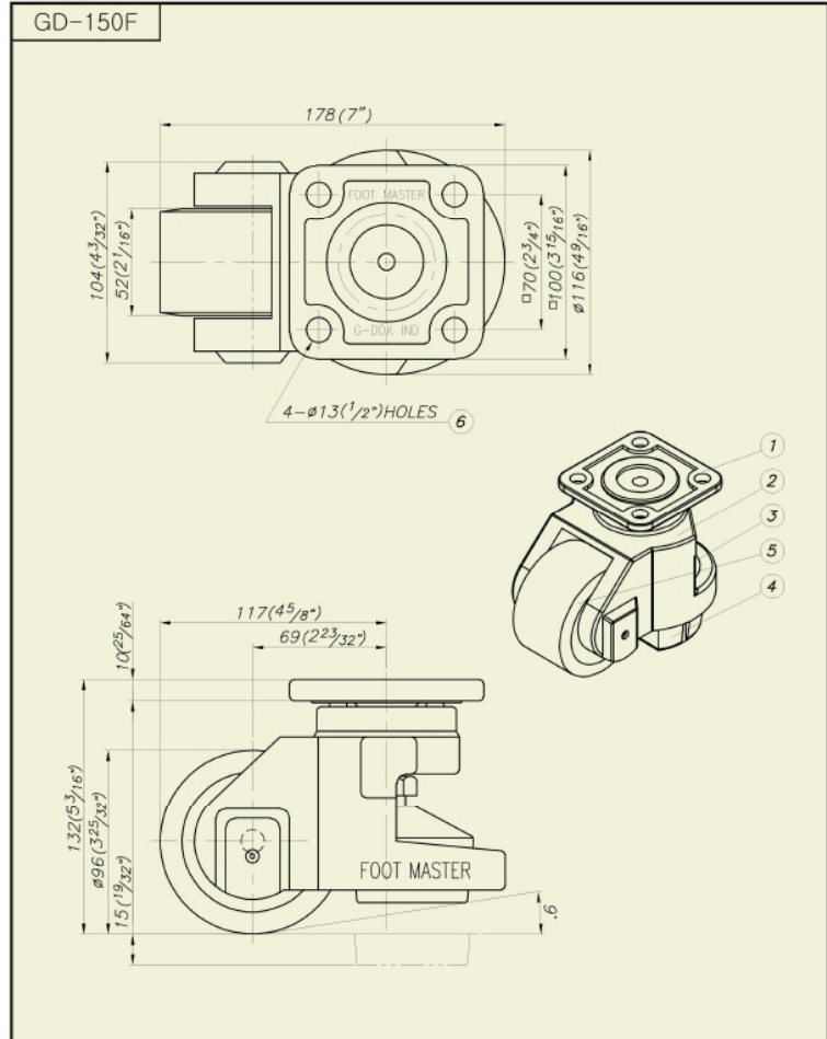
GD-150F-B (Wheel with ball bearing)
